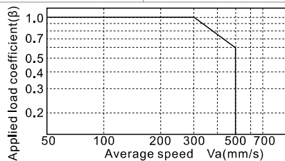
Fig 3 : Applied load coefficient (β)
