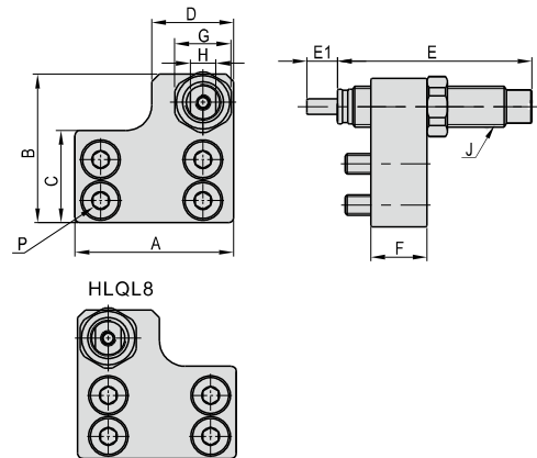
BF: Shock absorber(Retraction, for symmetrical)
