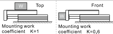
Fig 2 : Mounting work coefficient (K)
