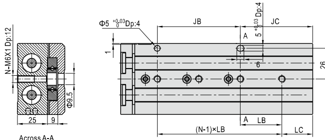
Across A-A
