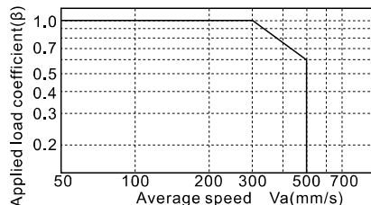
Fig 3 : Applied load coefficient (β)
