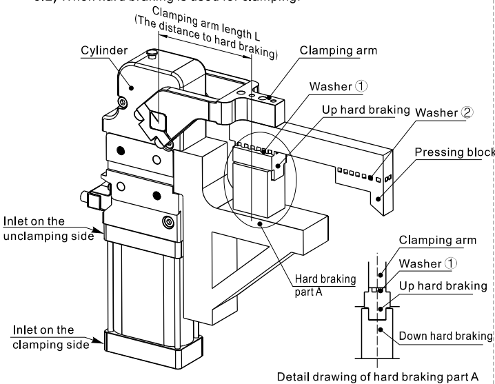
Detail drawing of hard braking part A
