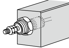
Embedded mounting (used for MPEF type)
