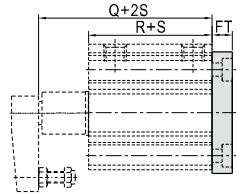
QCK□-FB(Taper type with clamp arm)
